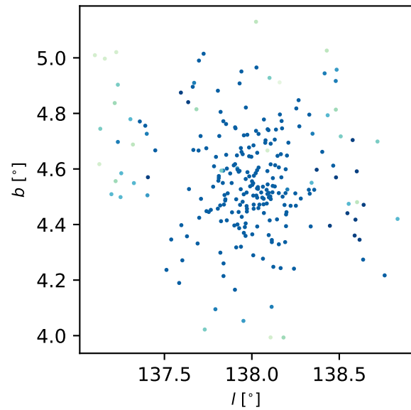
Trumpler 3
