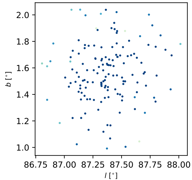
NGC 6991
