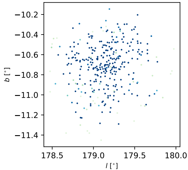
NGC 1750
