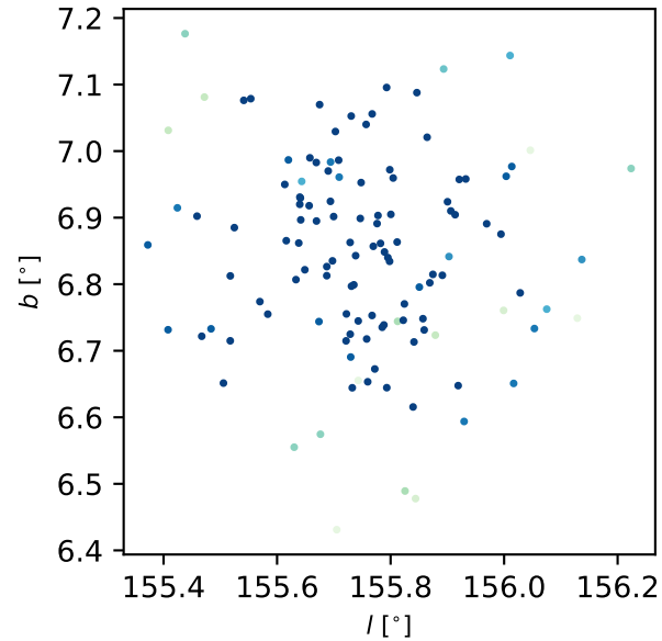
NGC 1708
