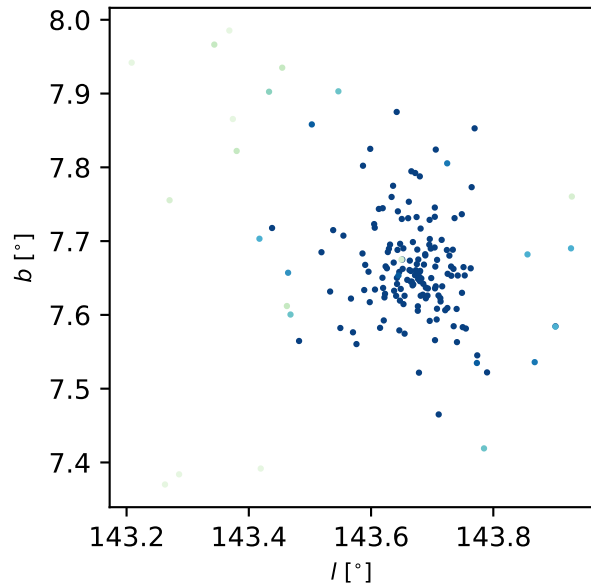
NGC 1502
