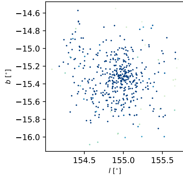
NGC 1342
