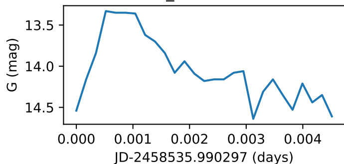
Star58_GWAC211016B
