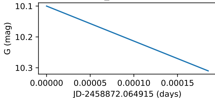
Star82_GWAC181212C
