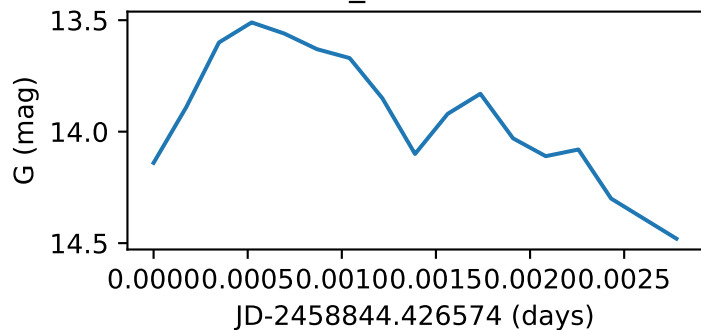
Star150_GWAC210413A
