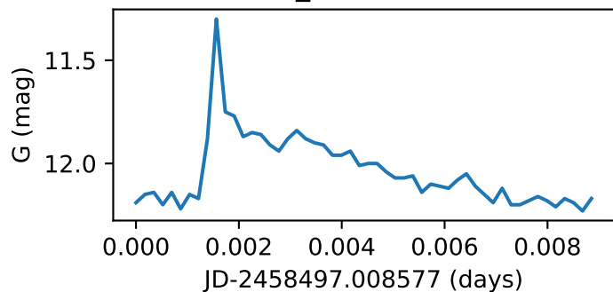
Star55_GWAC190221A
