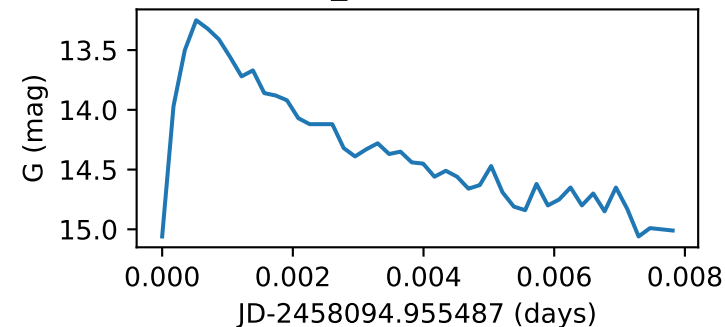
Star12_GWAC181129A
