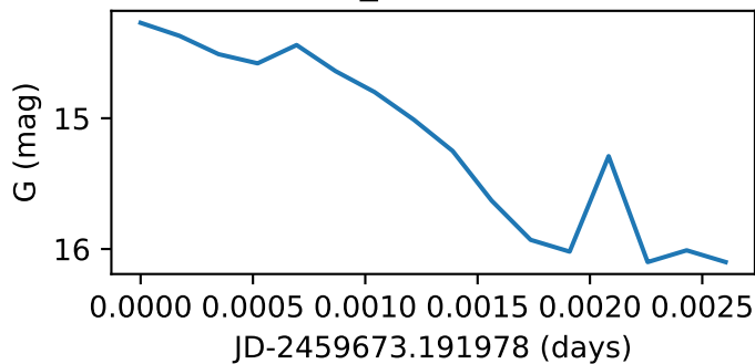
Star135_GWAC200319A
