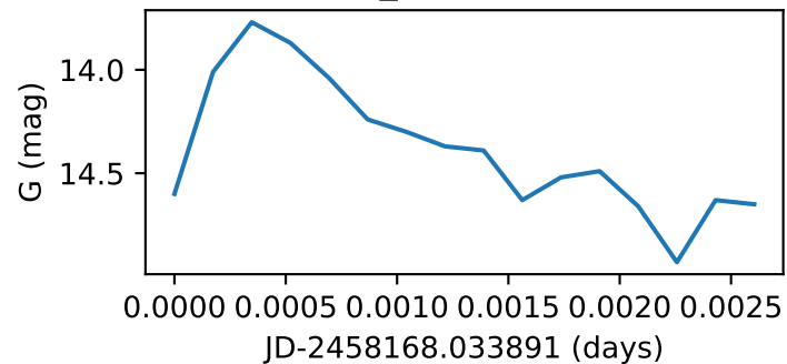
Star94_GWAC180218A
