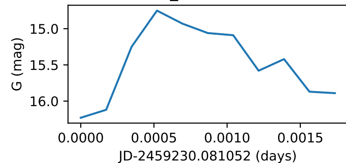
Star57_GWAC190121A
