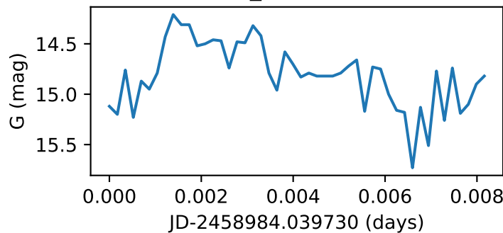
Star136_GWAC220523A
