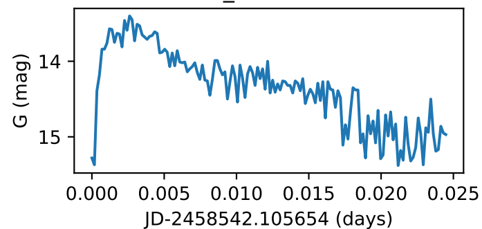
Star119_GWAC190227A
