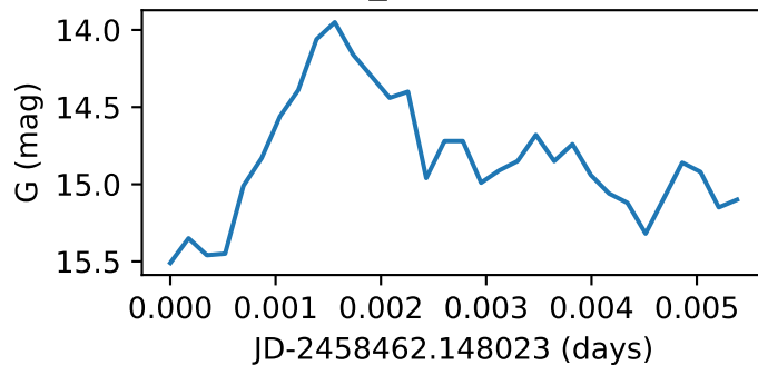
Star47_GWAC181209A
