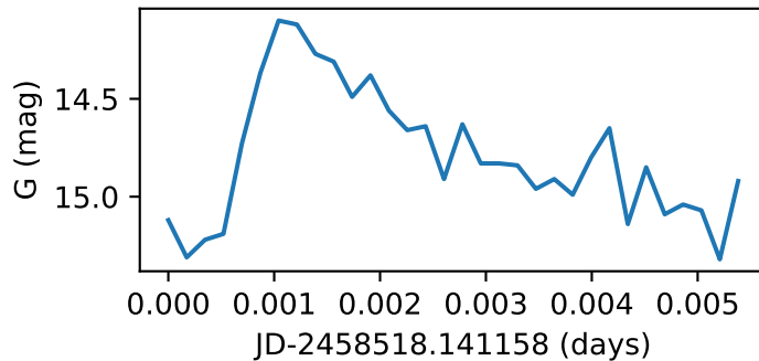
Star100_GWAC190324B
