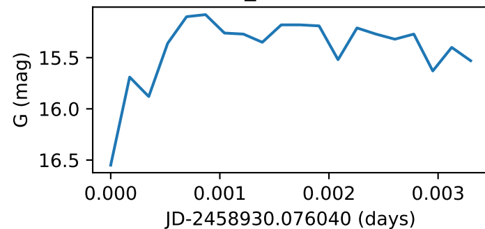
Star107_GWAC200321A
