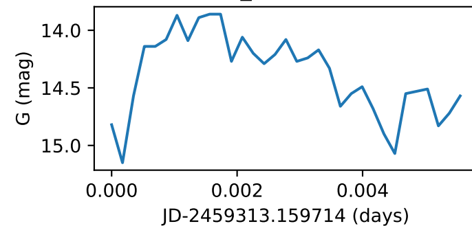
Star125_GWAC200317A
