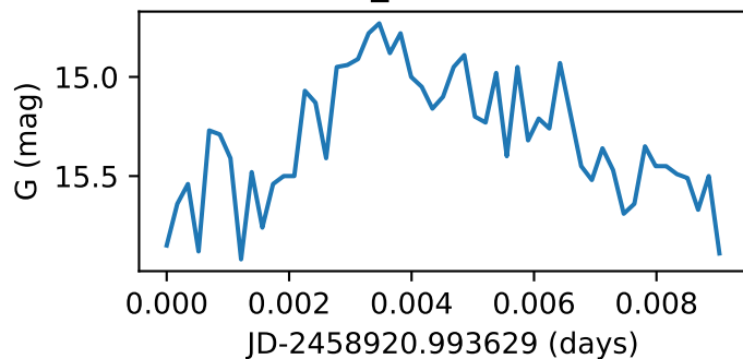
Star126_GWAC220204A
