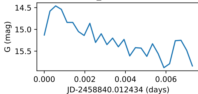
Star17_GWAC190124A
