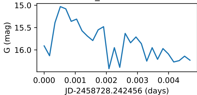
Star34_GWAC190901A
