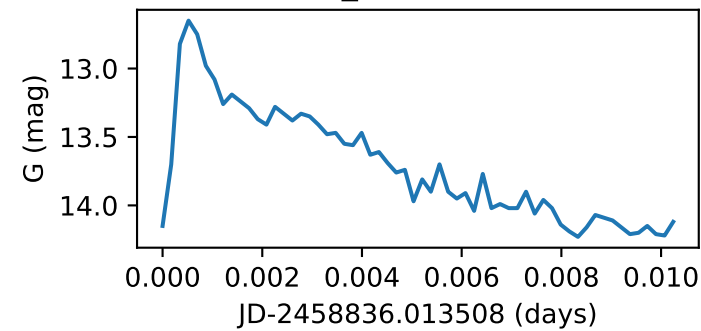
Star66_GWAC210209A
