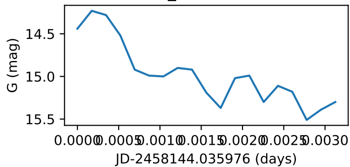
Star68_GWAC210218A
