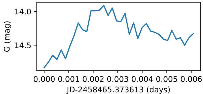
Star99_GWAC190105A
