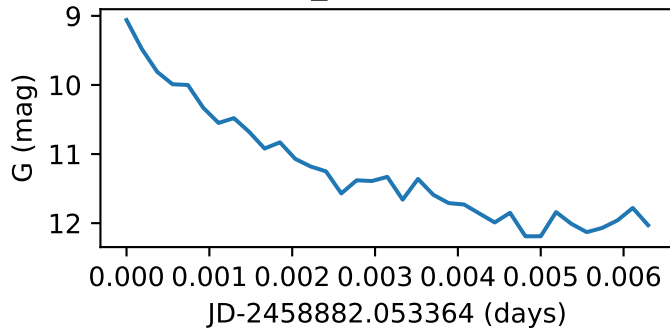
Star93_GWAC200202A
