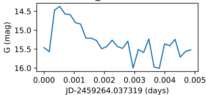
Star71_GWAC210208A
