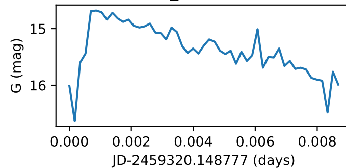
Star137_GWAC210416A
