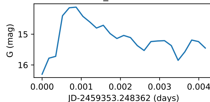
Star143_GWAC210518A
