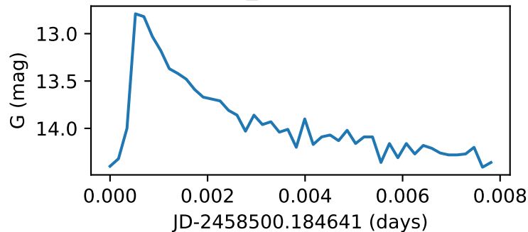
Star80_GWAC181028A
