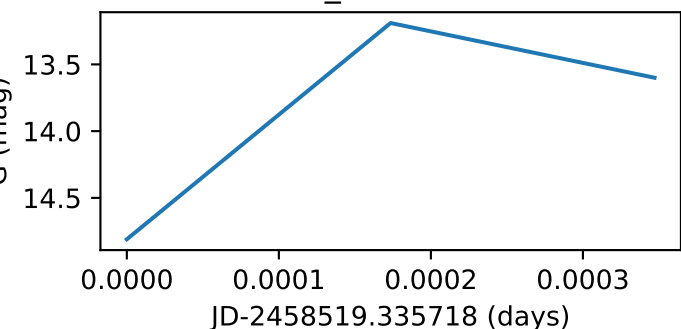
Star141_GWAC190204B
