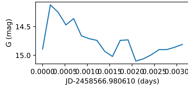
Star78_GWAC180207A
