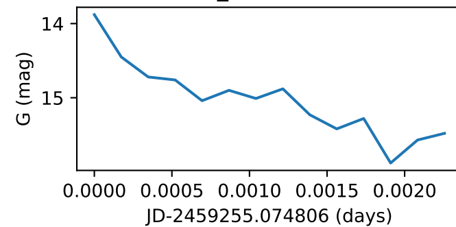
Star69_GWAC210414A
