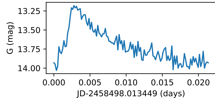
Star54_GWAC210115A
