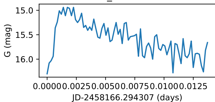
Star153_GWAC180216A
