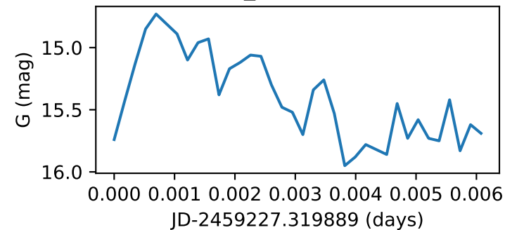
Star95_GWAC210112A
