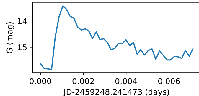
Star107_GWAC200321A
