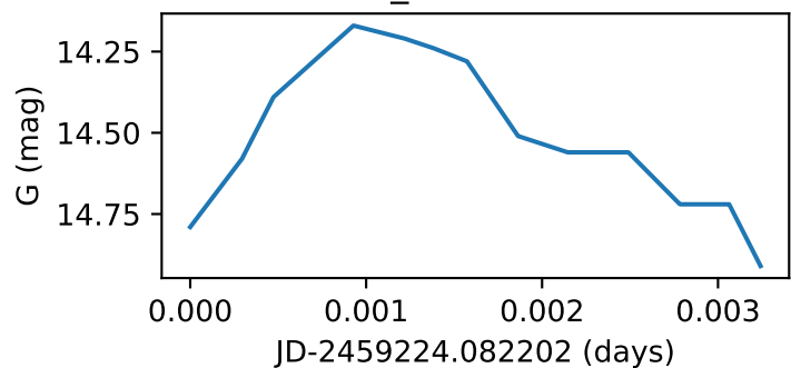
Star59_GWAC210109A
