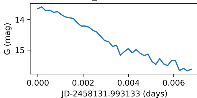
Star23_GWAC180113A
