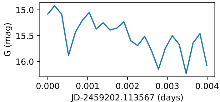
Star43_GWAC190121B
