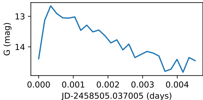
Star46_GWAC211212A
