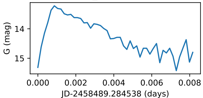
Star102_GWAC190206A
