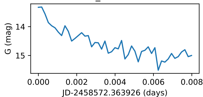
Star154_GWAC190329A
