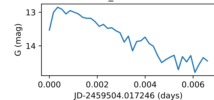
Star155_GWAC211016A
