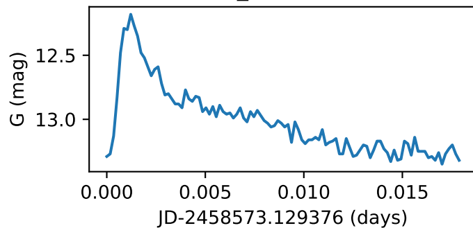
Star124_GWAC210217A
