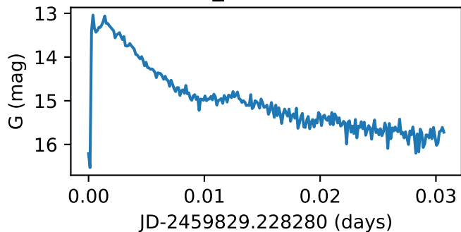
Star31_GWAC190203A
