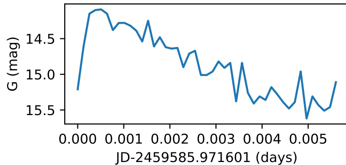
Star5_GWAC211124A
