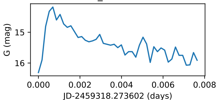
Star153_GWAC180216A
