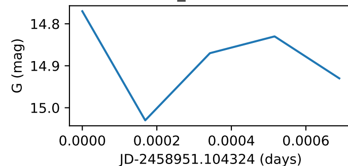
Star131_GWAC190414A
