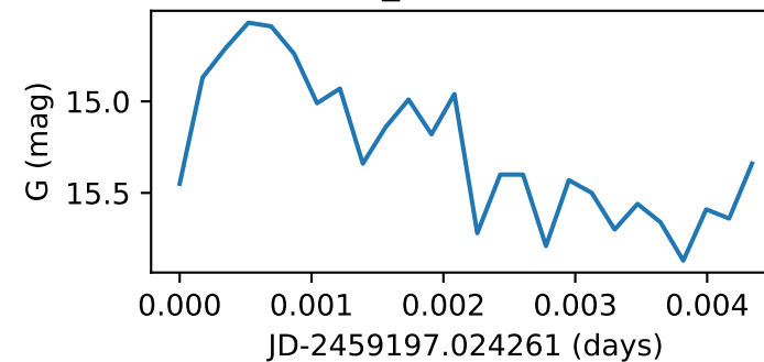
Star18_GWAC181208B
