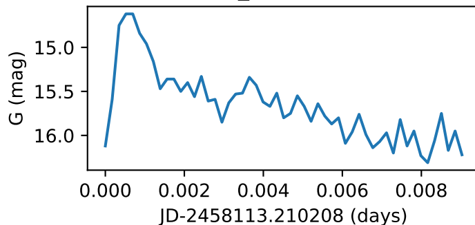
Star106_GWAC201216A
