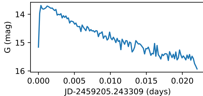
Star77_GWAC190116A
