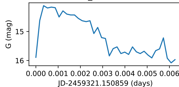
Star140_GWAC180210A
