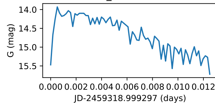
Star72_GWAC201217A
