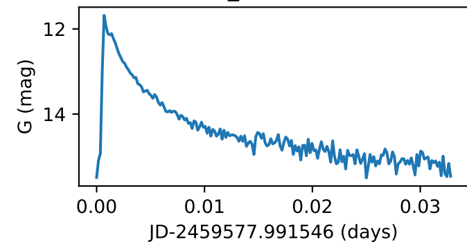
Star161_GWAC211229A
