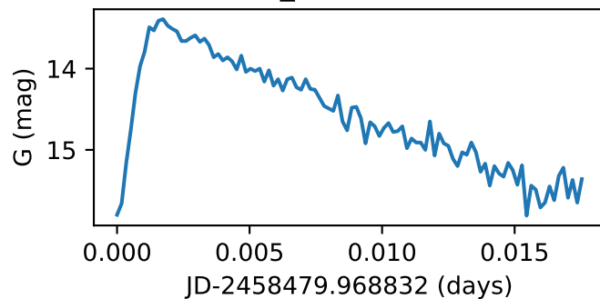
Star11_GWAC181227A
