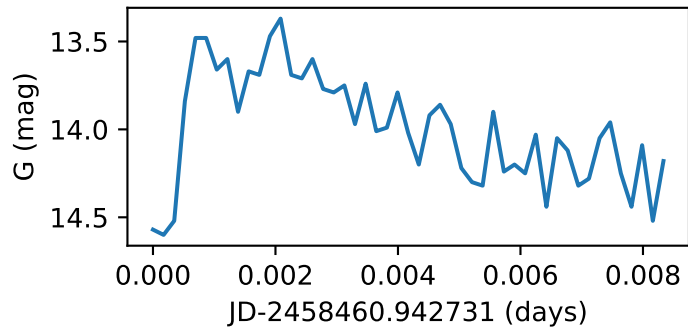
Star4_GWAC181206A
