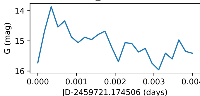
Star142_GWAC220521A
