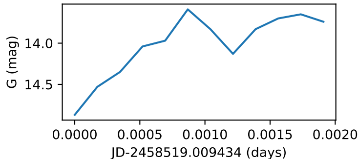
Star47_GWAC181209A
