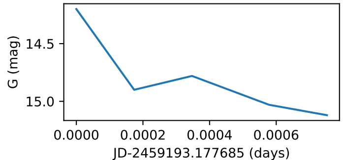
Star45_GWAC211231A
