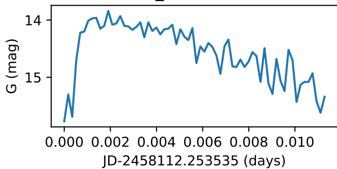
Star67_GWAC210121A
