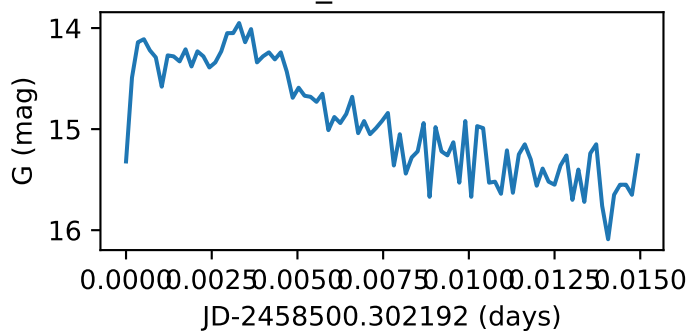
Star117_GWAC190116B
