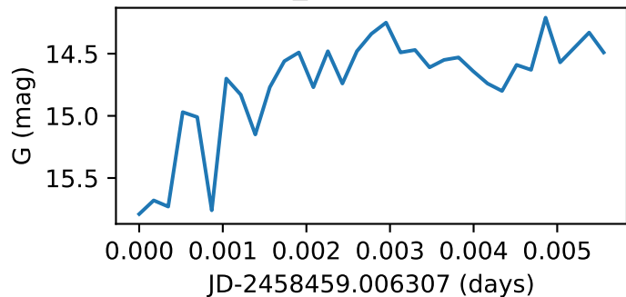
Star7_GWAC221210A
