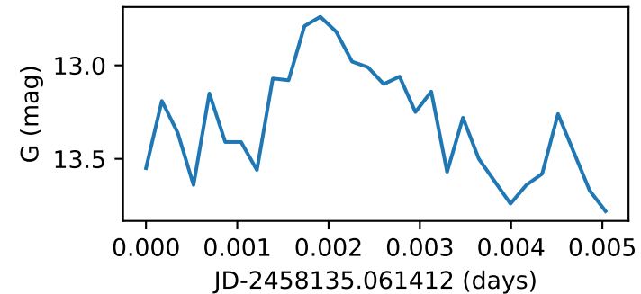
Star6_GWAC171221A
