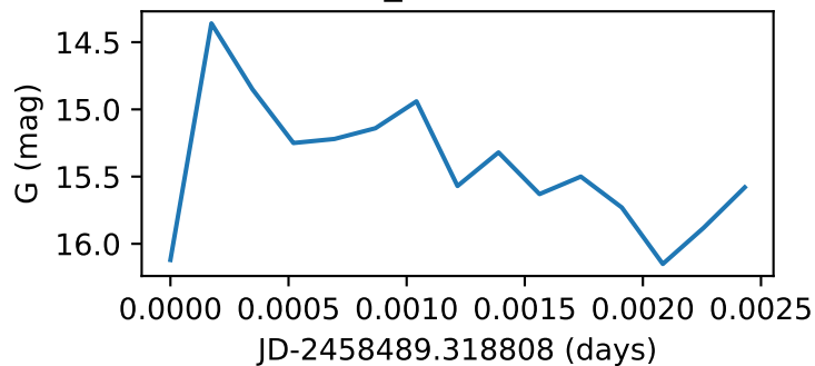
Star105_GWAC190105B
