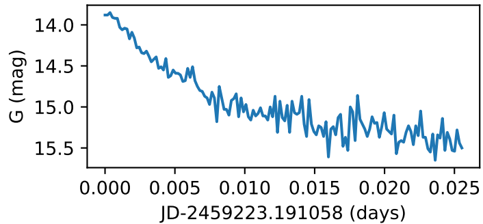
Star91_GWAC190113A
