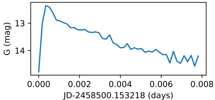
Star88_GWAC210108A
