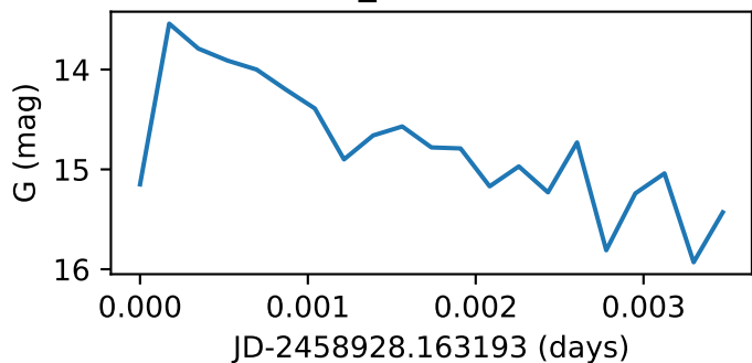
Star138_GWAC180209A
