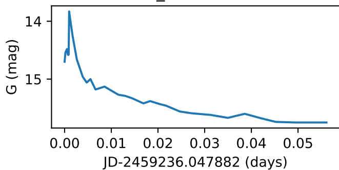
Star70_GWAC220209A
