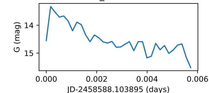
Star131_GWAC190414A
