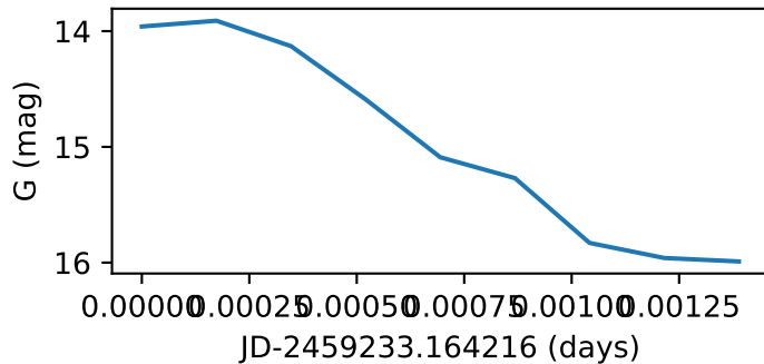
Star76_GWAC201113A
