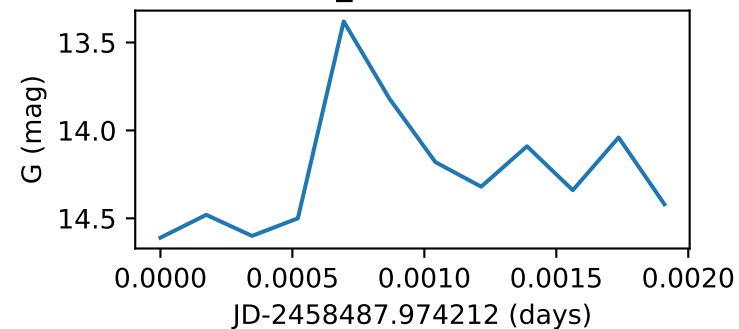
Star33_GWAC181212B
