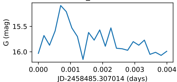
Star117_GWAC190116B
