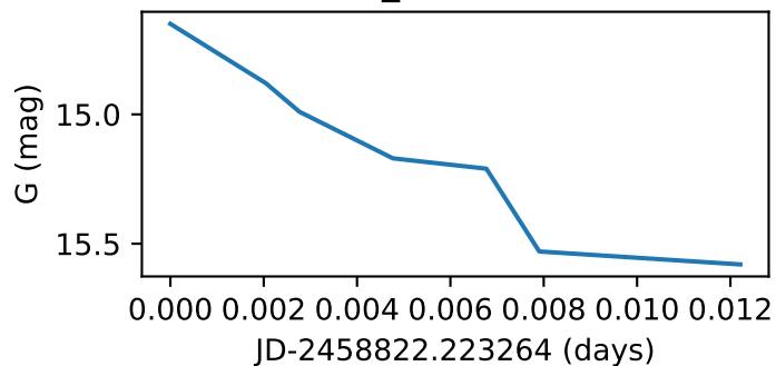
Star114_GWAC190101B
