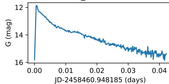
Star21_GWAC181225A
