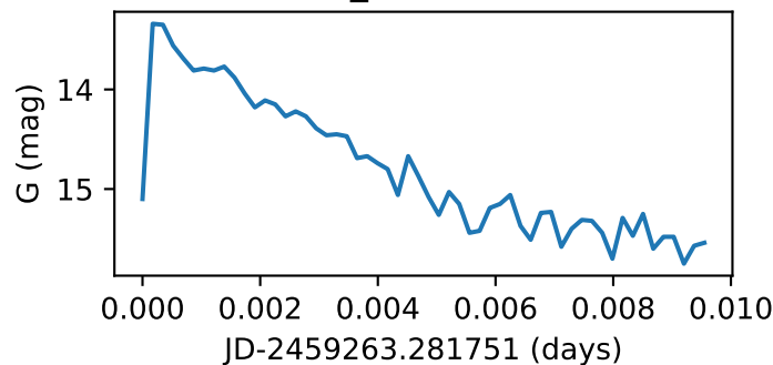
Star127_GWAC210430A
