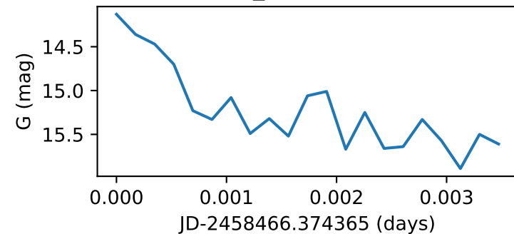
Star84_GWAC181213C
