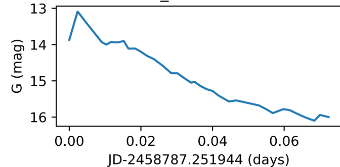
Star60_GWAC191030A
