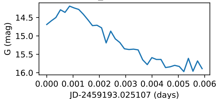
Star11_GWAC181227A
