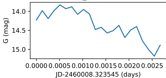
Star147_GWAC191226A
