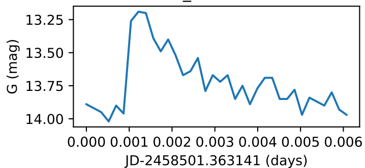
Star118_GWAC190117B
