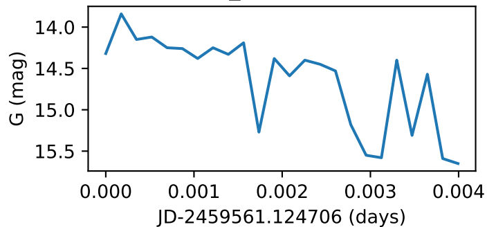
Star46_GWAC211212A
