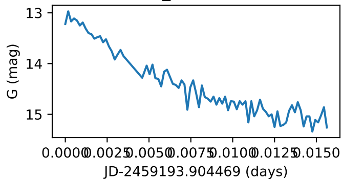
Star162_GWAC201202A
