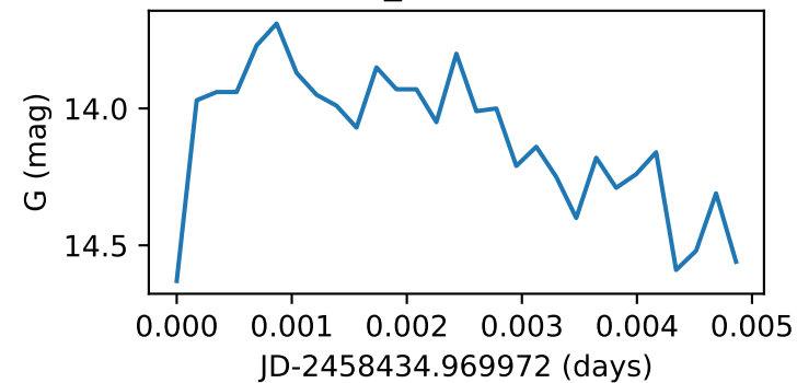
Star161_GWAC211229A
