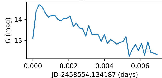
Star104_GWAC210202A
