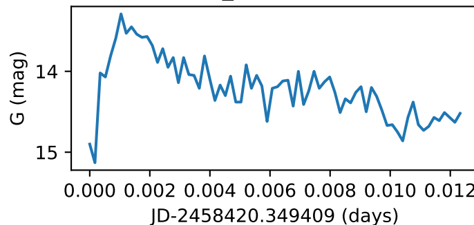
Star83_GWAC210210A
