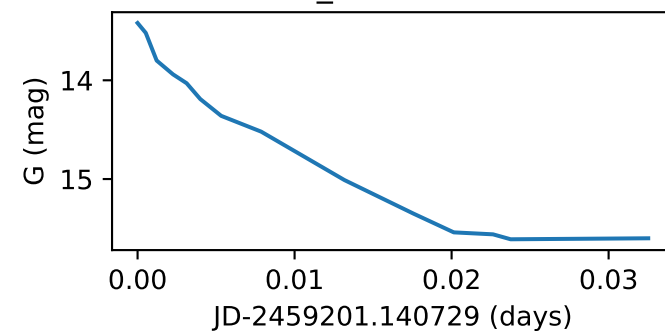
Star72_GWAC201217A
