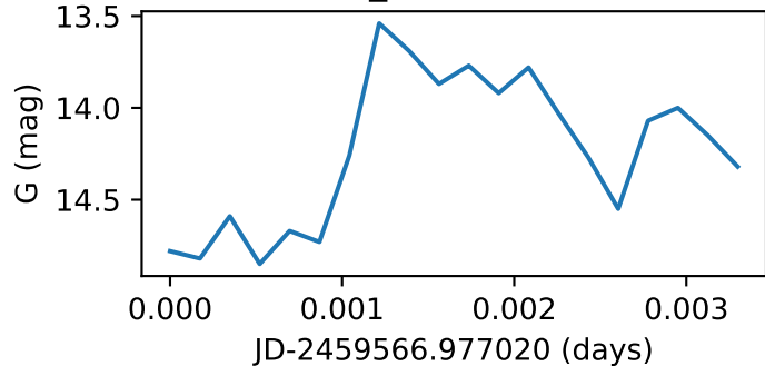
Star10_GWAC211218A
