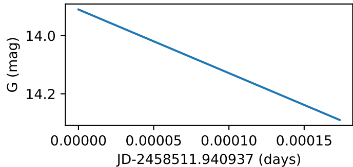
Star40_GWAC201218A
