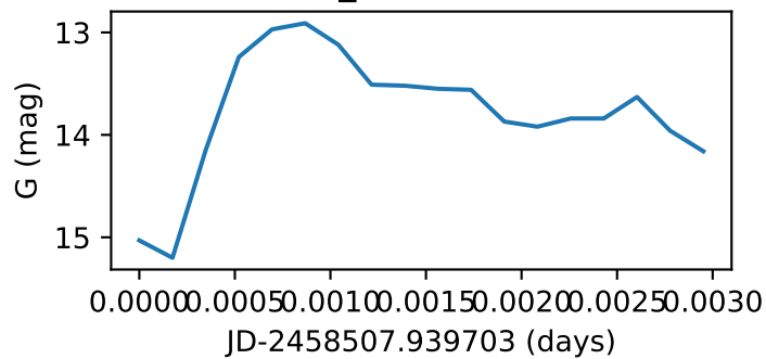
Star20_GWAC190120A
