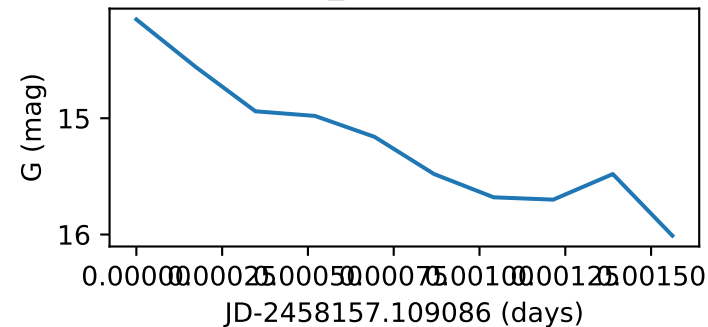
Star81_GWAC181213B
