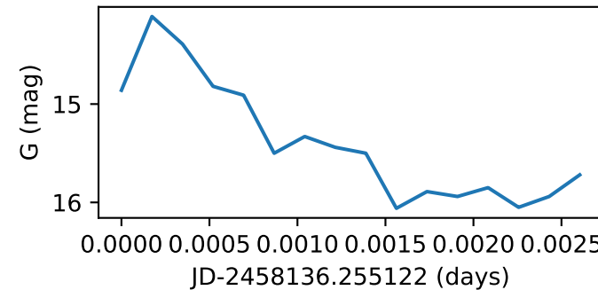
Star101_GWAC190311A
