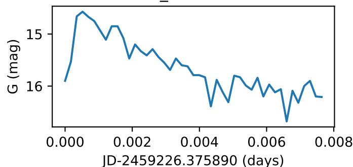
Star130_GWAC210111A
