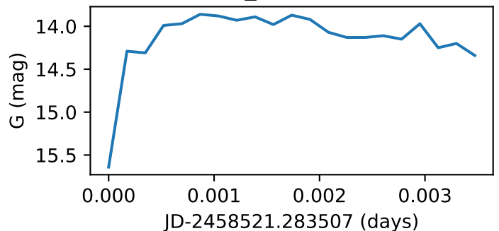
Star105_GWAC190105B
