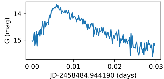
Star42_GWAC201209C
