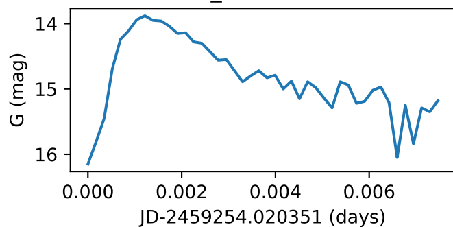
Star71_GWAC210208A
