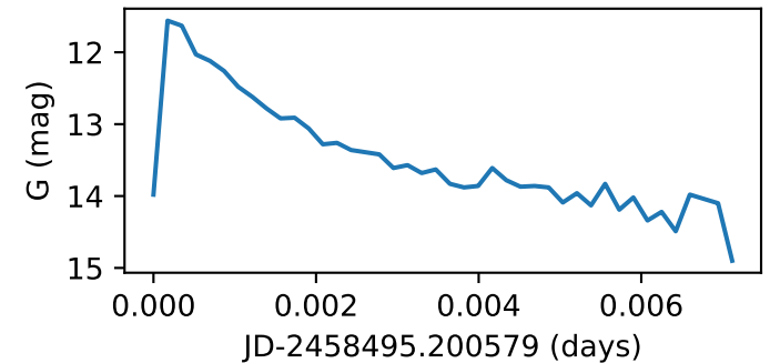
Star90_GWAC201220A
