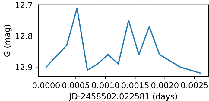
Star53_GWAC181212A
