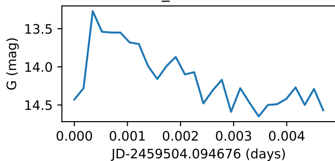
Star58_GWAC211016B
