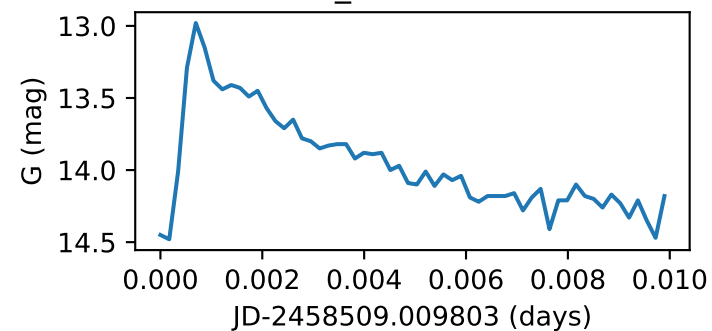
Star36_GWAC190125D
