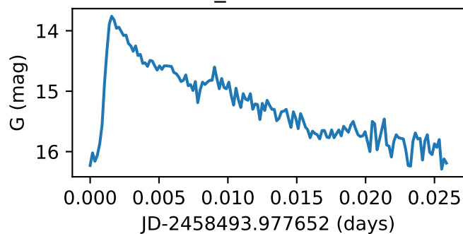
Star35_GWAC190110A
