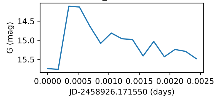
Star128_GWAC200411A
