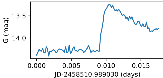
Star41_GWAC190125E
