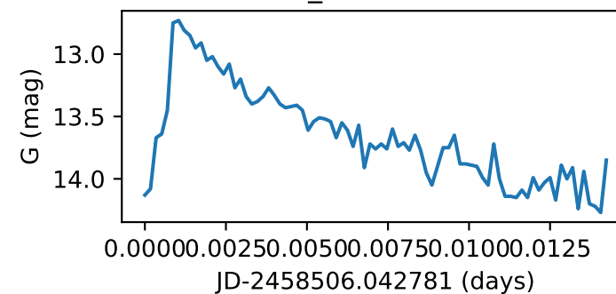
Star24_GWAC190122A
