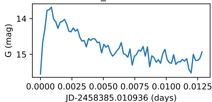
Star154_GWAC190329A
