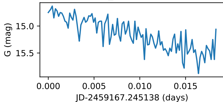
Star79_GWAC200123A
