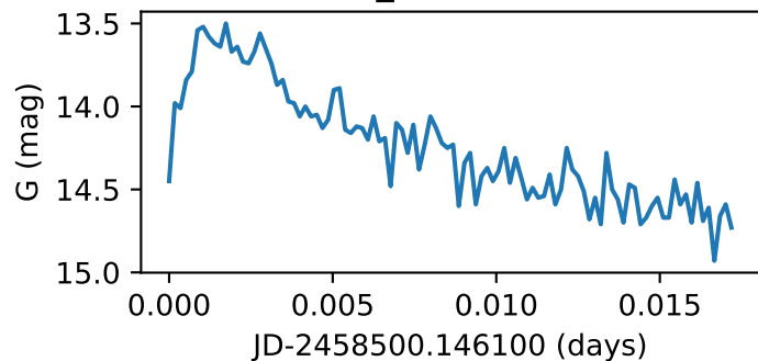
Star115_GWAC181219A
