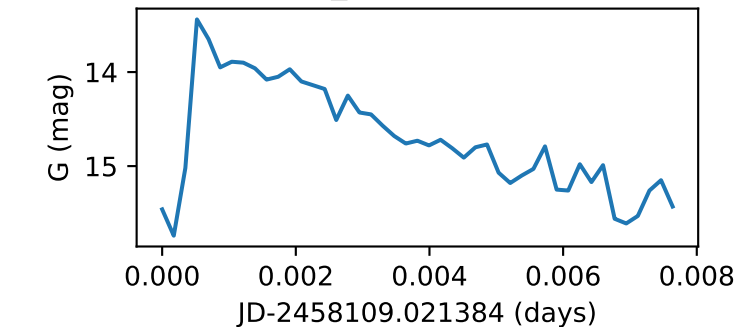
Star9_GWAC171207A
