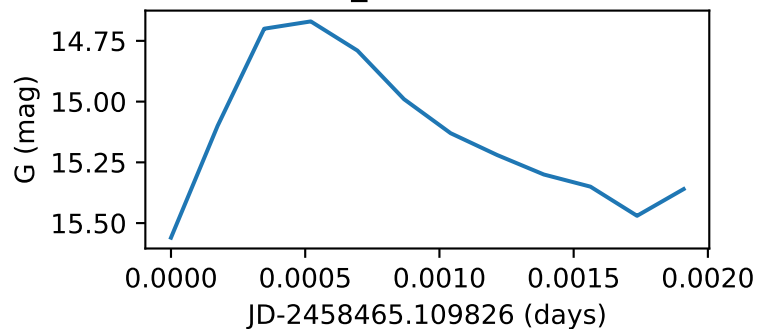
Star56_GWAC190113B
