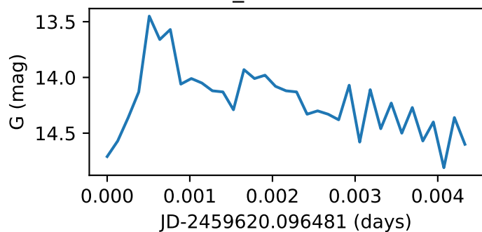
Star70_GWAC220209A
