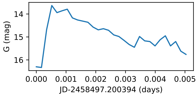
Star93_GWAC200202A
