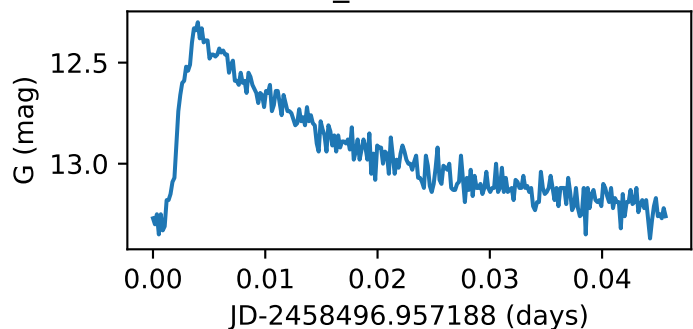
Star59_GWAC210109A
