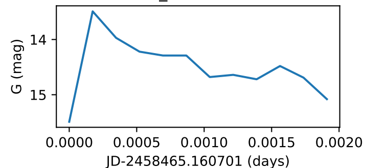
Star36_GWAC190125D
