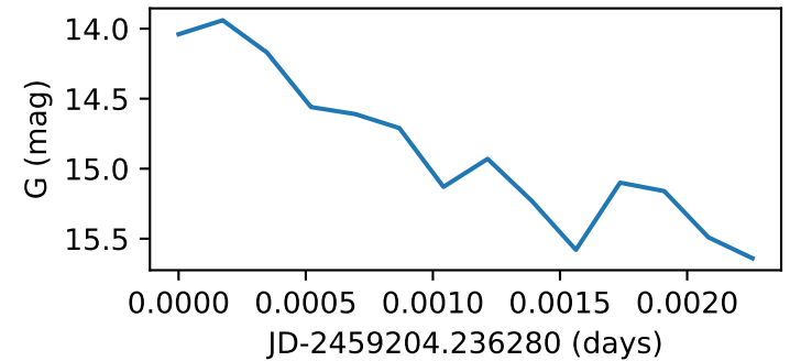
Star93_GWAC190125B
