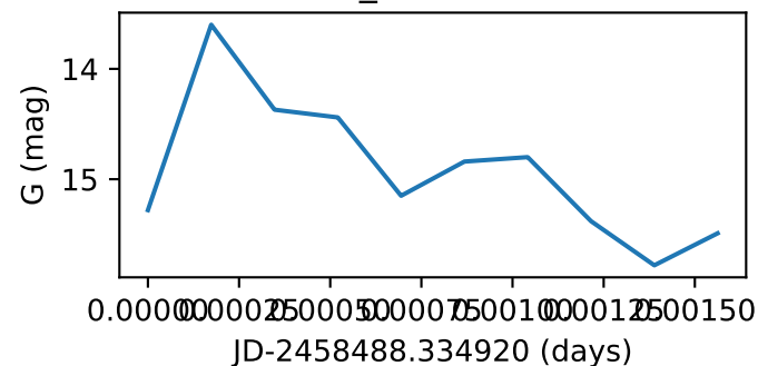
Star119_GWAC190227A
