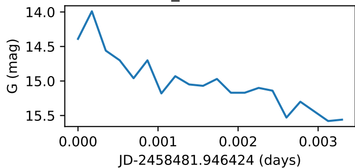
Star22_GWAC201019A
