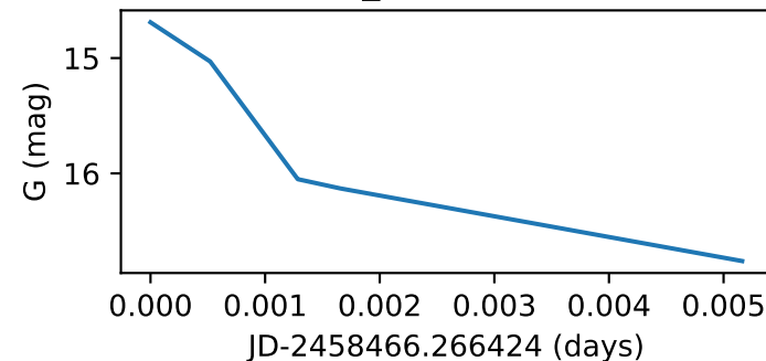
Star84_GWAC181213C
