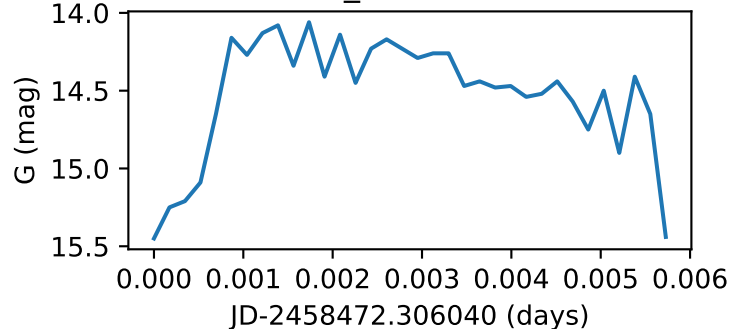
Star118_GWAC190117B
