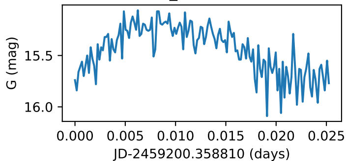
Star106_GWAC201216A
