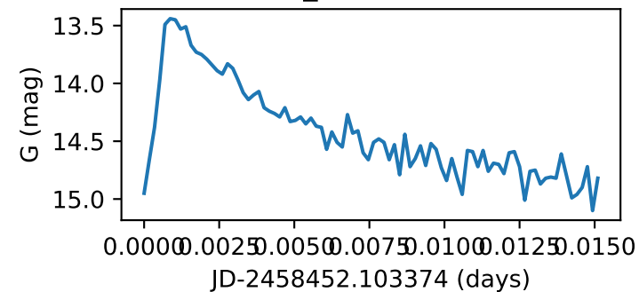
Star12_GWAC181129A
