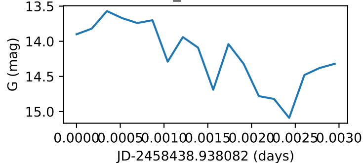
Star151_GWAC180923A
