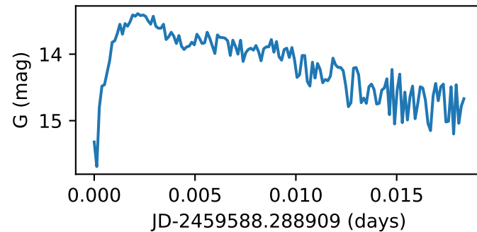
Star94_GWAC180218A
