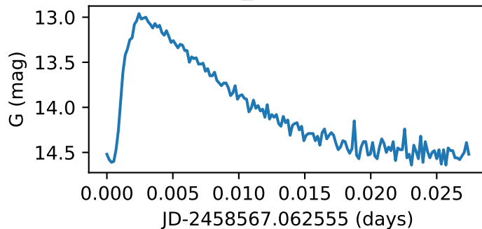
Star103_GWAC171225A
