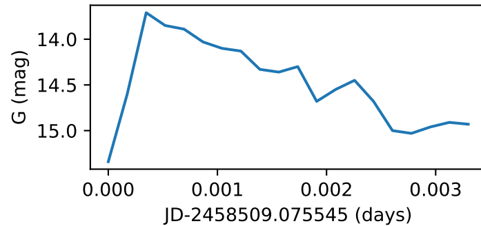
Star92_GWAC220108A
