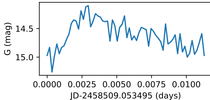
Star44_GWAC190204A
