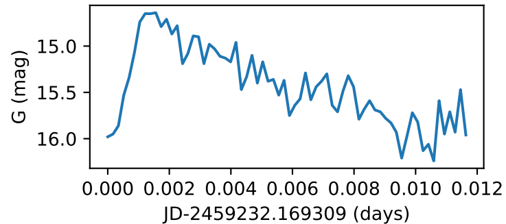
Star89_GWAC190125A
