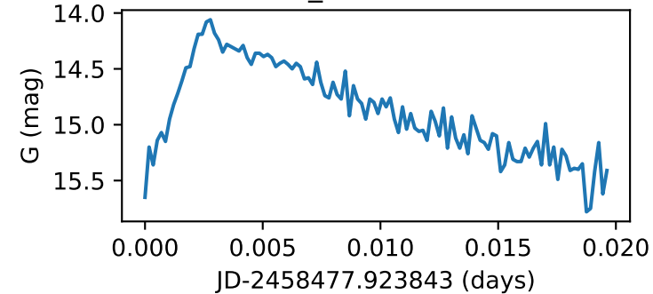
Star24_GWAC190122A
