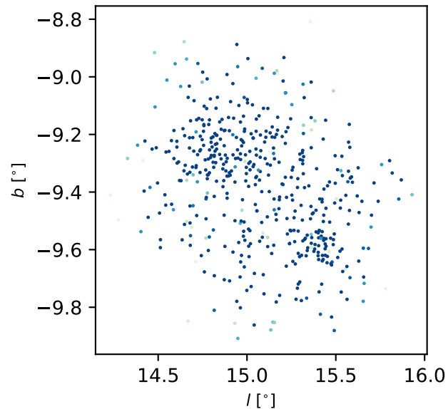
Collinder 394
