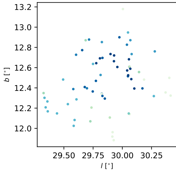
Collinder 359
