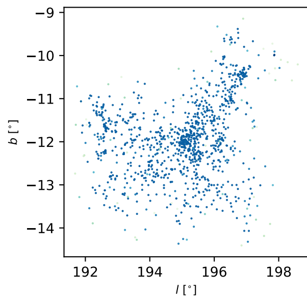
Collinder 69
