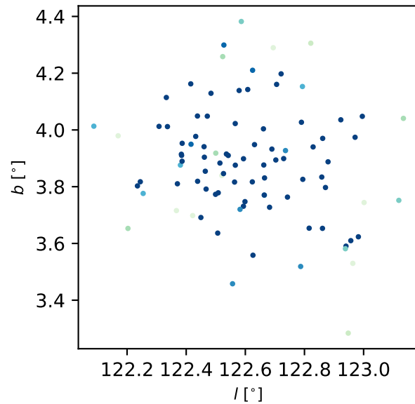
COIN - Gaia 1
