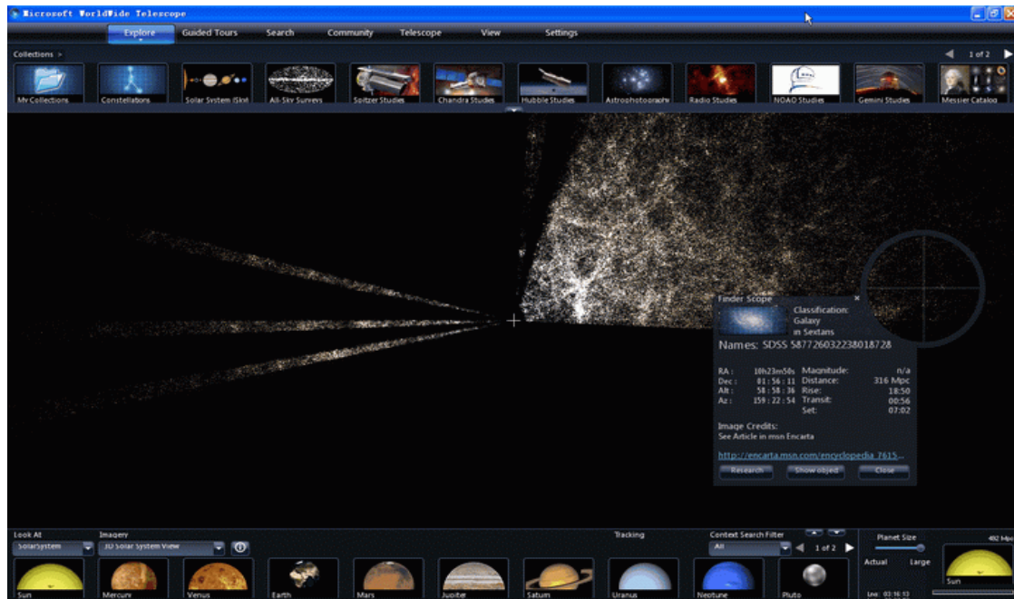
Figure 1. SDSS huge dataset displayed in WWT with further information
