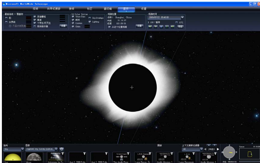
Figure 2. Total solar eclipse simulated by WWT
