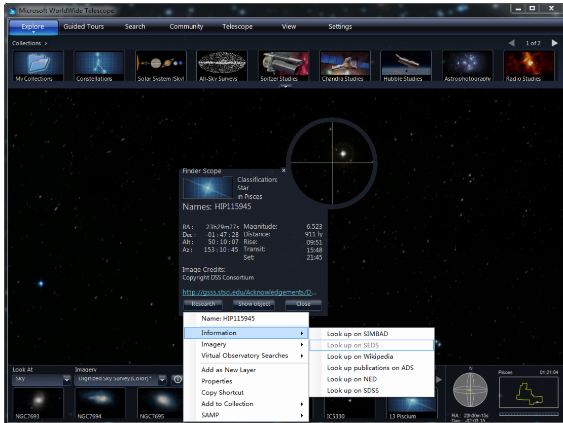
Fig 5. Further links to professional databases to provide rich information for an object
